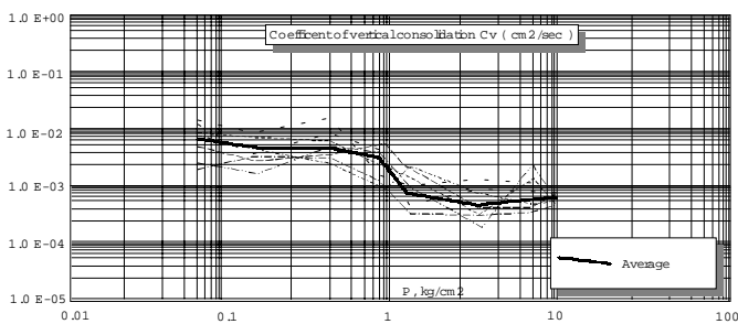
Fig 2 : preliminary soil investigation results
