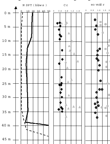
Fig 10 : Soil improvement comparative results
